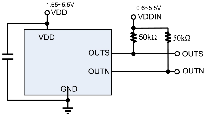
Figure 1, Typical Application Circuit of AS1820AOD
