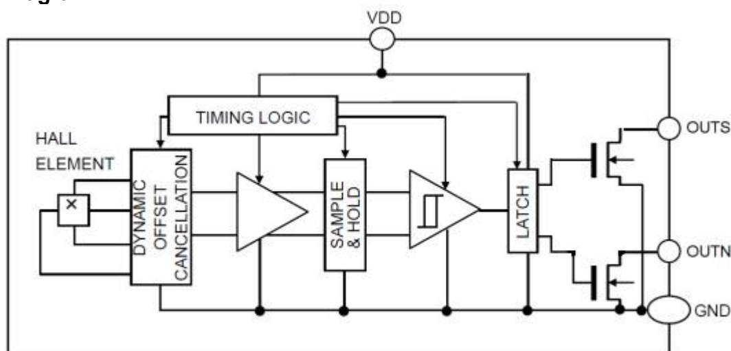
Figure 2, Block Diagram of AS1820AOD
