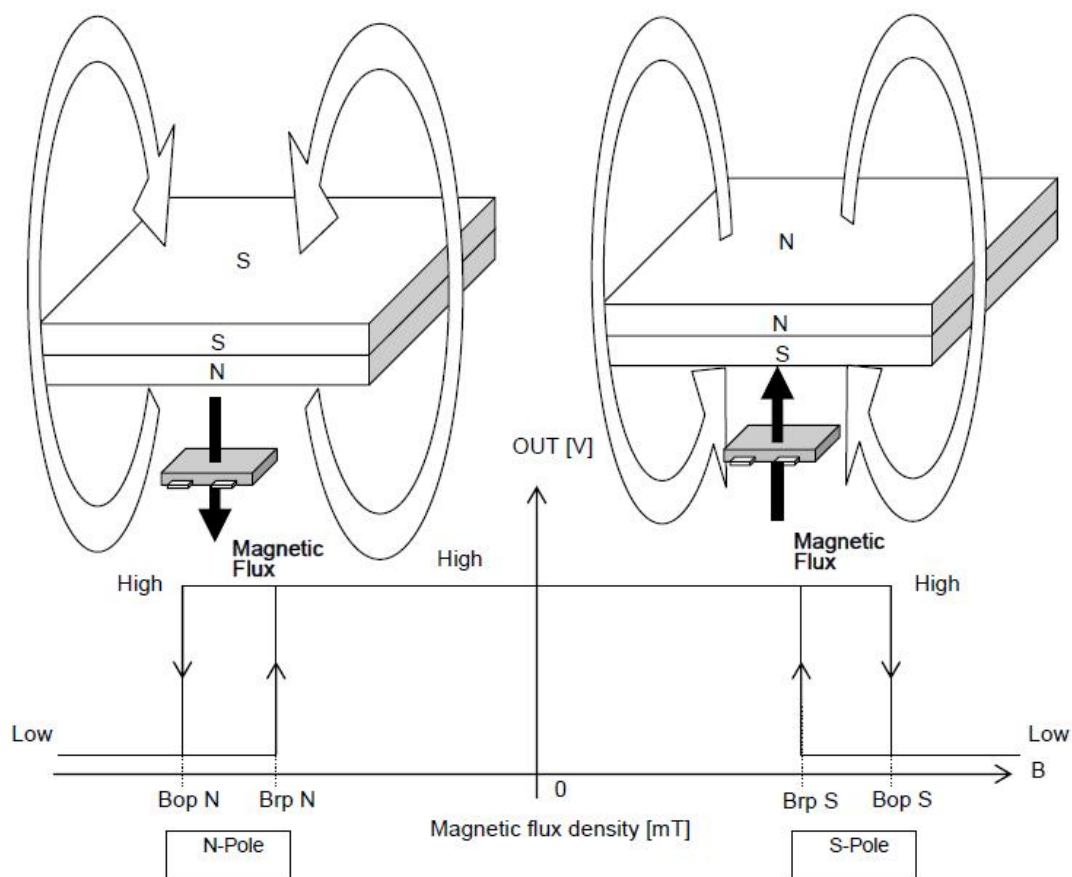
Figure 3, Magnetic Operation Characteristic of AS1820AOD
